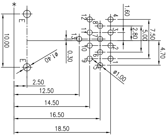
L:1.6 DIMENSIONS OF PC BOARD HOLES TOLERANCE: ±0.05(PRINTED-TOP VIEW)
