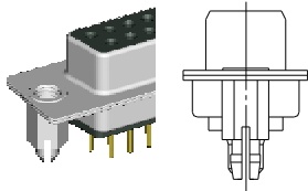
K TYPE WITH #4-40UNC IN THE REAR SHELL USE RIVET AS BOARDLOCK
